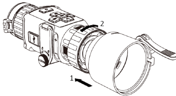
Figure 2-4 Install Adapter
